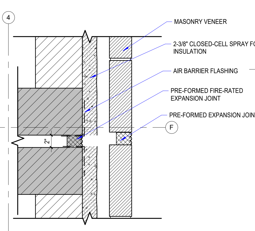
15 AREA B EJ - HIGH ROOF A180 1 1/2" = 1'-0"
