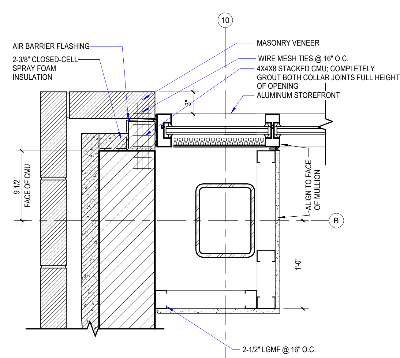
26 DETAIL A180 1 1/2" = 1'-0"
