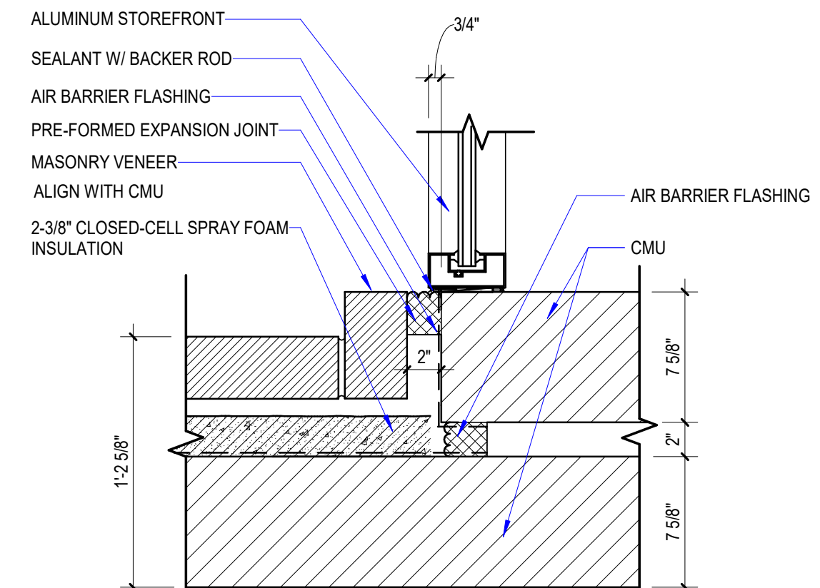
24 DETAIL A180 1 1/2" = 1'-0"
