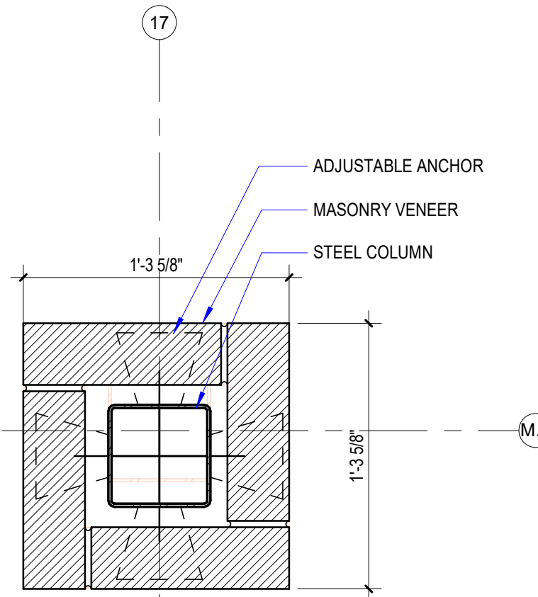
1 DETAIL A180 1 1/2" = 1'-0"
