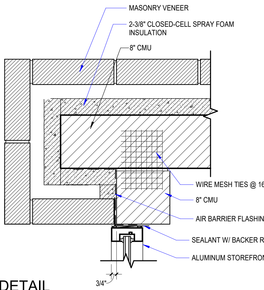
2 DETAIL A180 1 1/2" = 1'-0"
