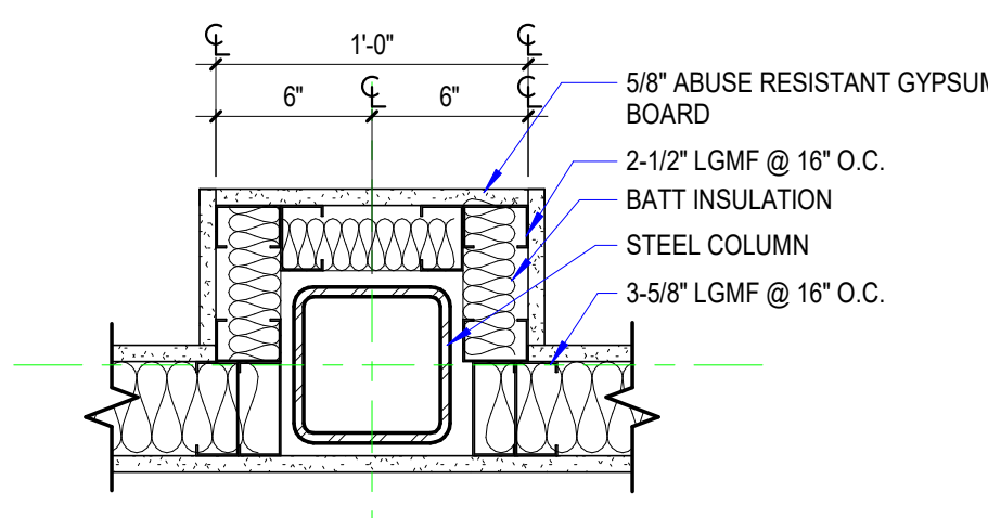
5 TYP. COL WRAP @ WALL A180 1 1/2" = 1'-0"
