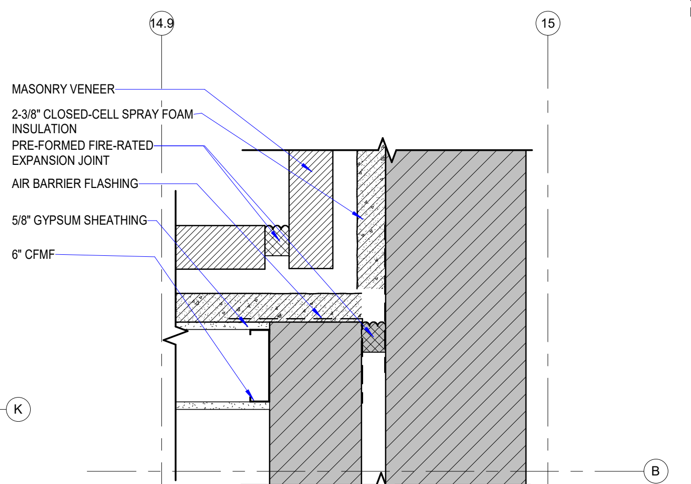
14 DETAIL A180 1 1/2" = 1'-0"
