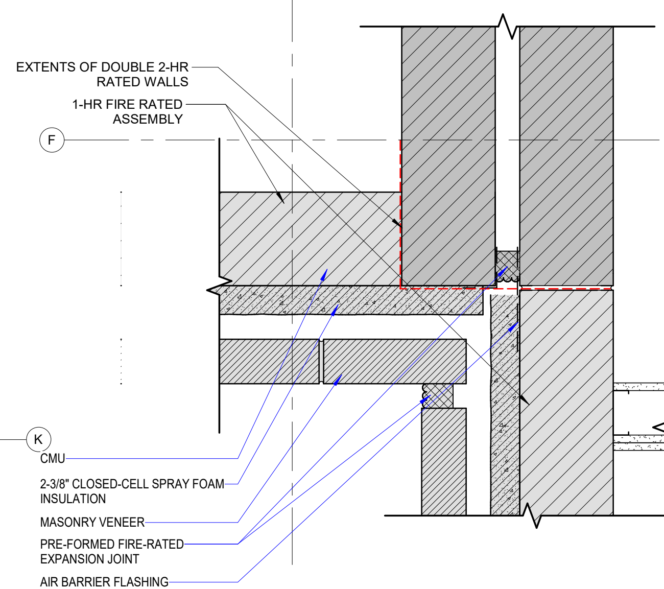
19 DETAIL A180 1 1/2" = 1'-0"
