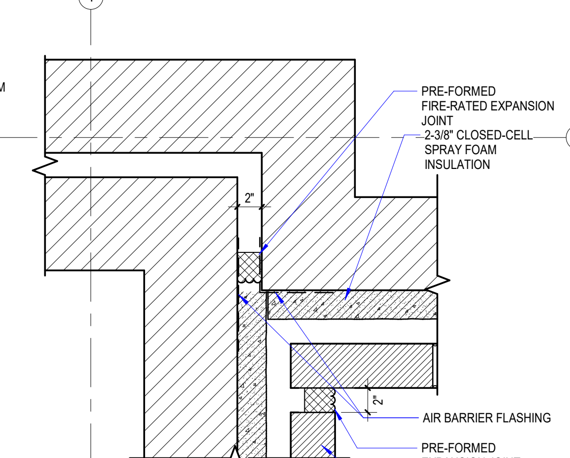
16 DETAIL A180 1 1/2" = 1'-0"
