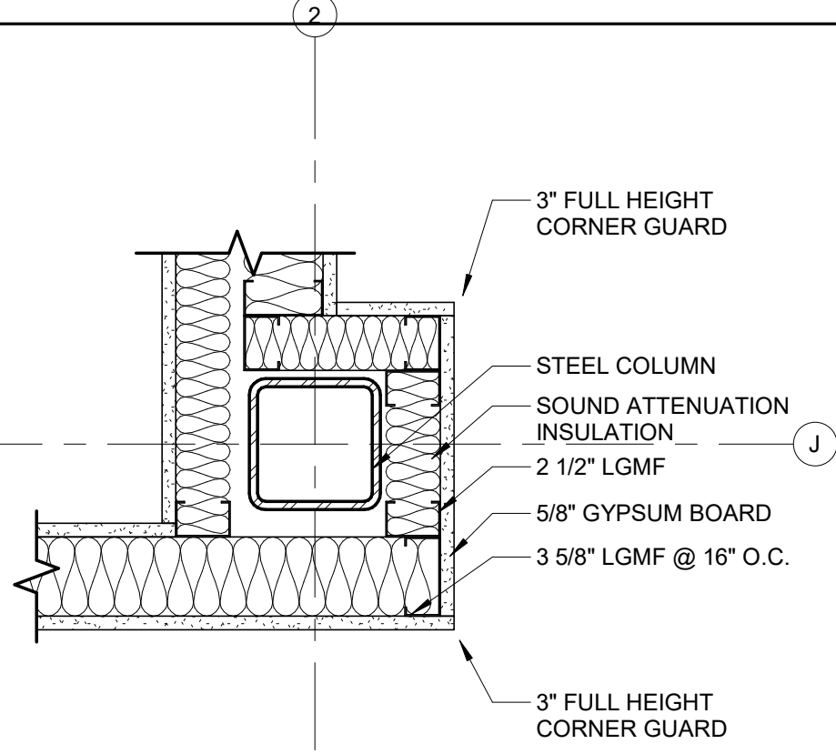
1 DETAIL A180 1 1/2" = 1'-0"
