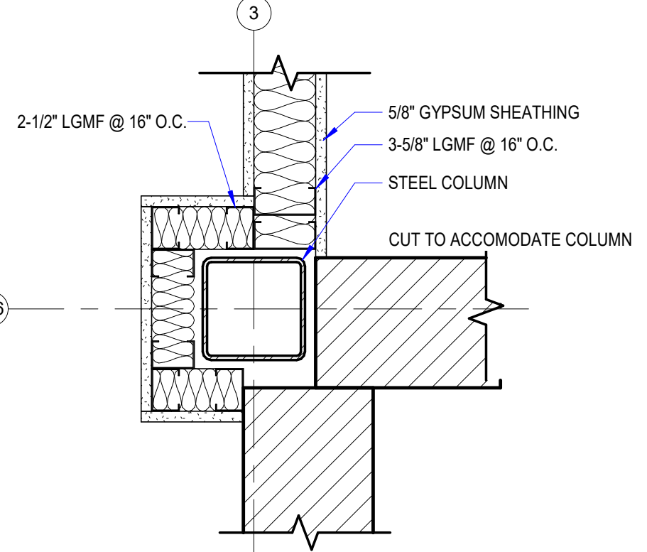
11 DETAIL A180 1 1/2" = 1'-0"
