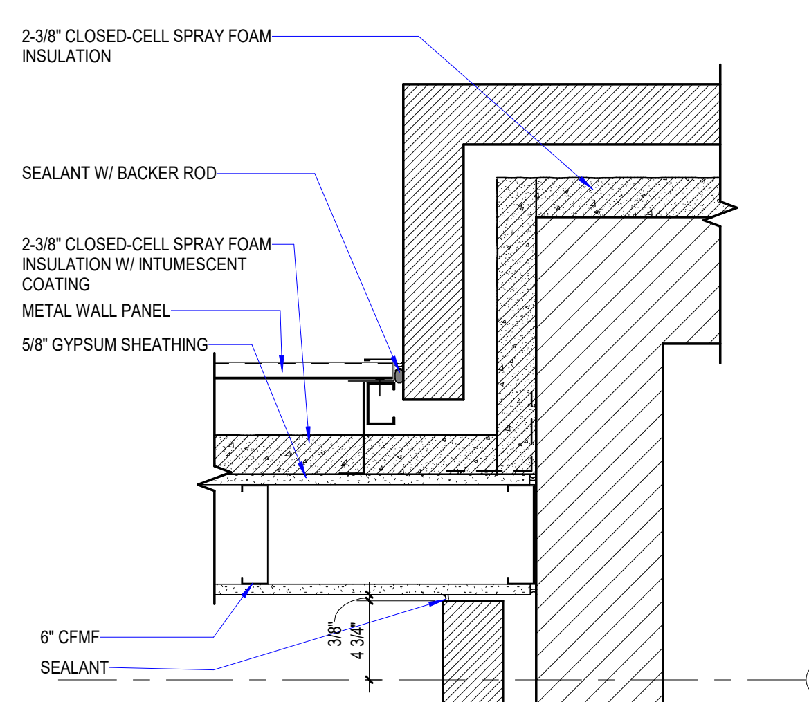
12 DETAIL A180 1 1/2" = 1'-0"
