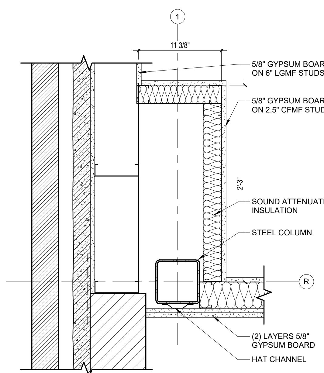
27 DETAIL A180 1 1/2" = 1'-0"
