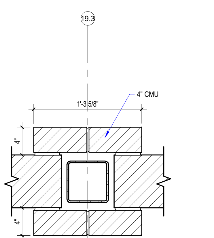
18 DETAIL A180 1 1/2" = 1'-0"
