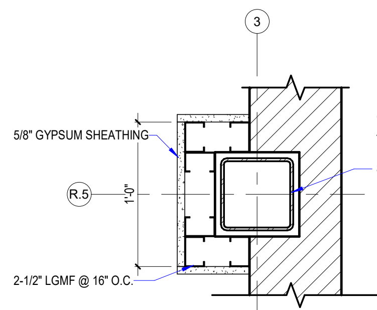
4 DETAIL A180 1 1/2" = 1'-0"
