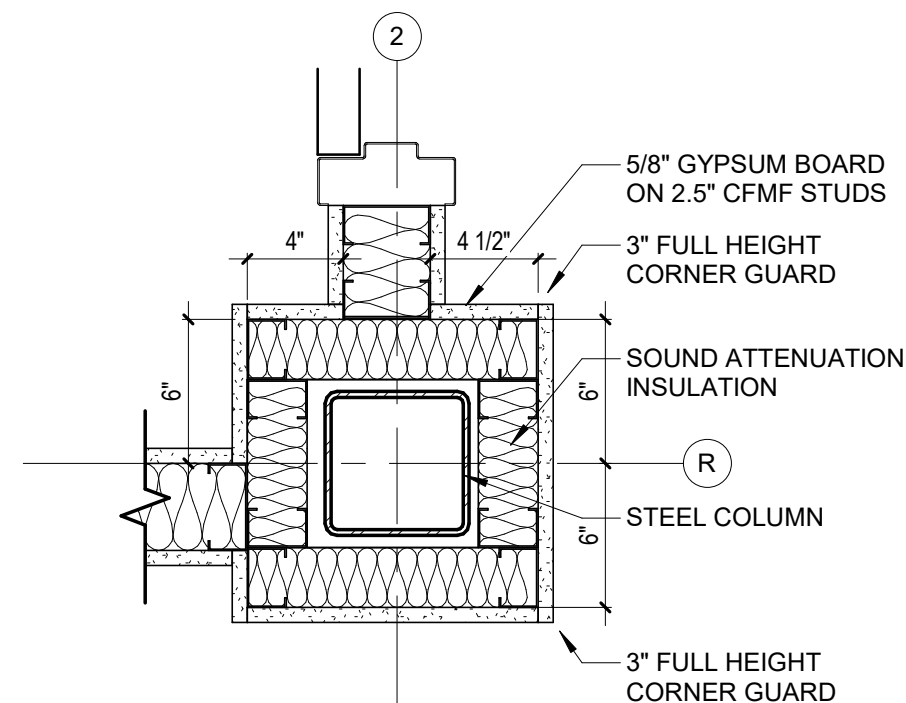
2 DETAIL A180 1 1/2" = 1'-0"
