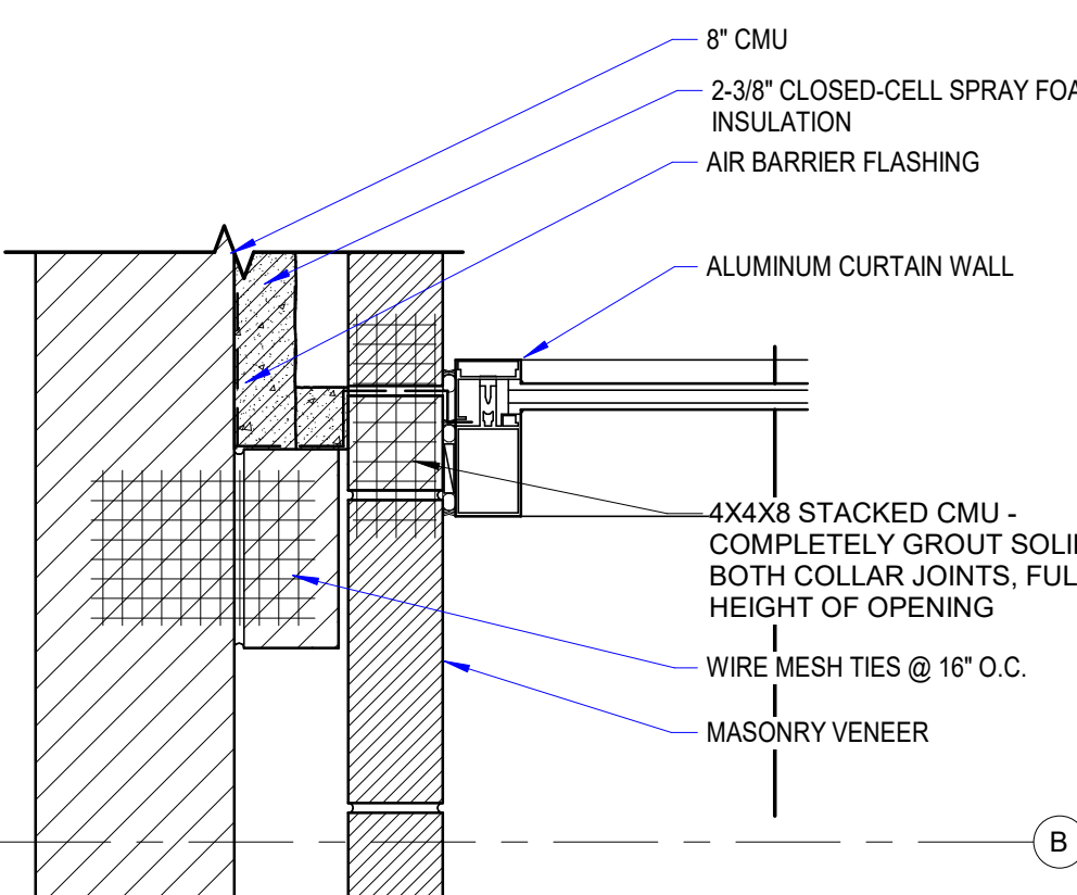
22 DETAIL A180 1 1/2" = 1'-0"
