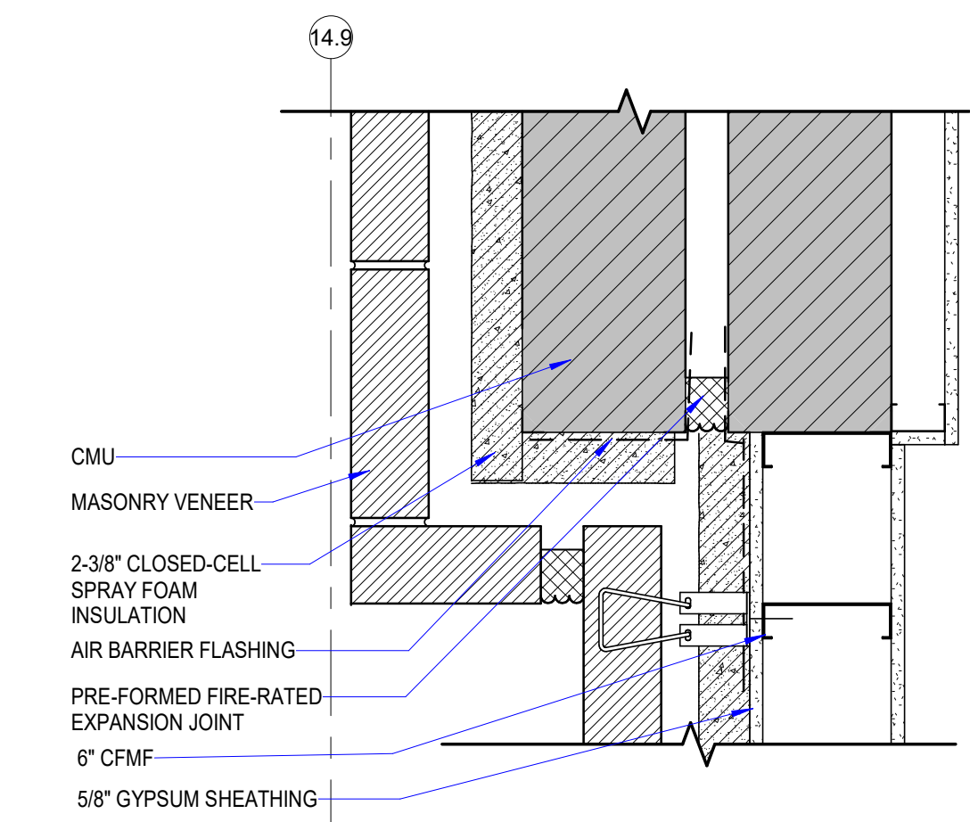
21 DETAIL A180 1 1/2" = 1'-0"
