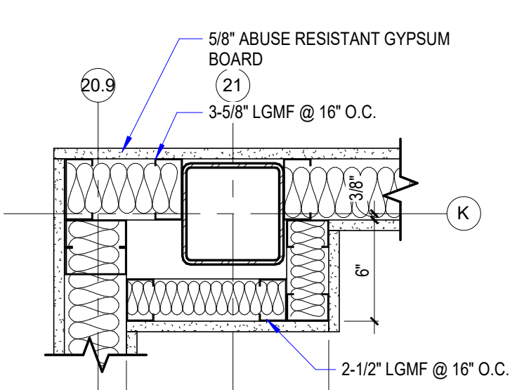
23 DETAIL A180 1 1/2" = 1'-0"
