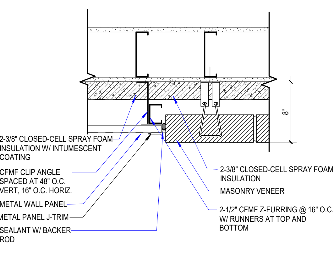
20 DETAIL A180 1 1/2" = 1'-0"
