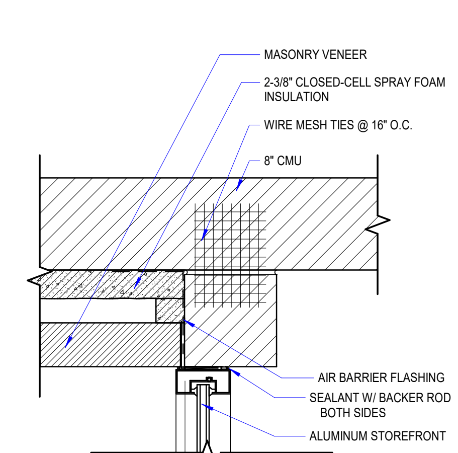
17 DETAIL A180 1 1/2" = 1'-0"
