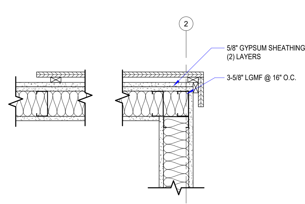
6 DETAIL A180 1 1/2" = 1'-0"
