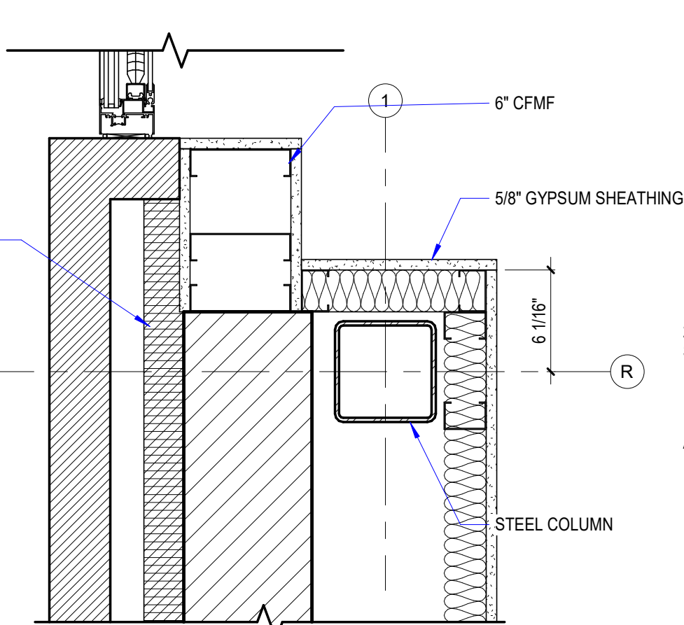
9 DETAIL A180 1 1/2" = 1'-0"
