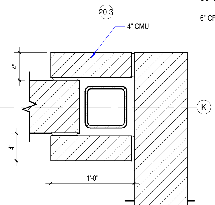
13 Detail 305 A180 1 1/2" = 1'-0"
